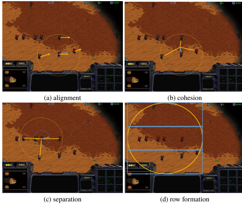
Fig. 3: The augmented screenshots (a) to (c) depict the steering urges as defined by Reynolds' flocking algorithm [19]. Based on these urges, formations emerge such as the one in (d).
